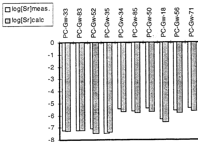
Figure 6. Comparison between Sr concentrations calculated by applying a codissolution approach and Sr concentrations measured in Morro do Ferro.
