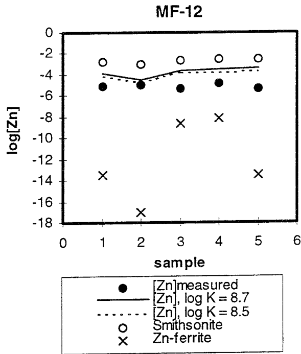
Figure 2.b) Results obtained in borehole MF-12
