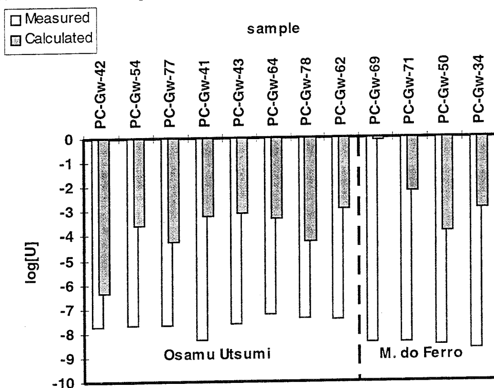
Figure 9. Calculated U concentrations by assuming equilibrium with U_3O_8 versus measured U content in the selected groundwaters.
