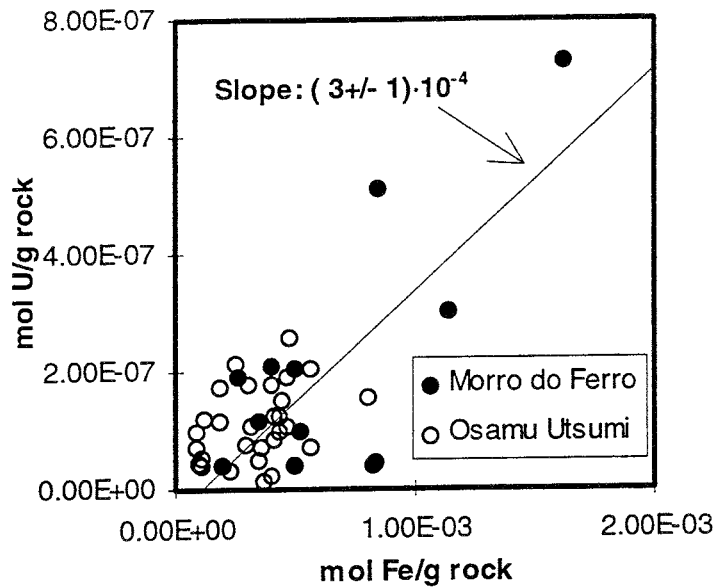
Figure 10. Uranium versus Iron content in the host rock of Poços de Caldas.
