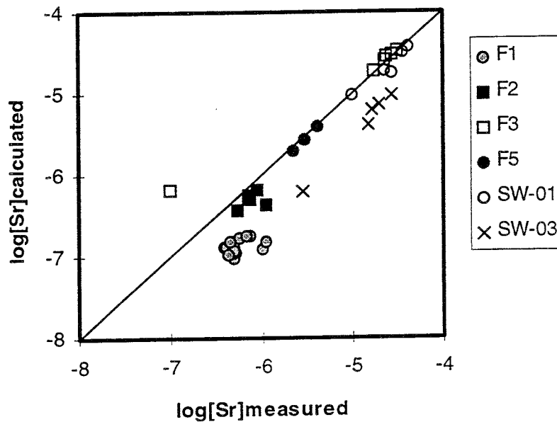
Figure 8. Correlation between the calculated and the measured concentrations in Osamu Utsumi mine.
