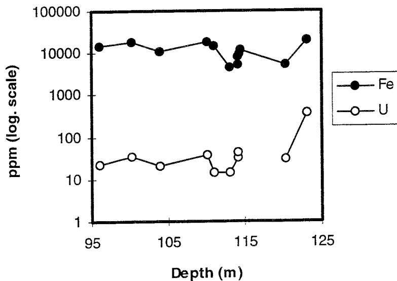
Figure 11. Variations in U and Fe concentrations with depth in borehole F1 (Osamu Utsumi mine)
